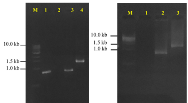
Fig. 2 Confirmation of the pEX-ANCB vector construction
