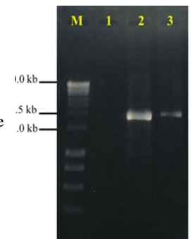
Fig. 5 Examination of the AN3860-CBM20 presence in the recombinant A. oryzae chromosome using PCR. 1: Negative control, distilled water; 2: Positive control, pEX-ANCB; 3: Genome template of selective clone. M: 1kb Ladder.
