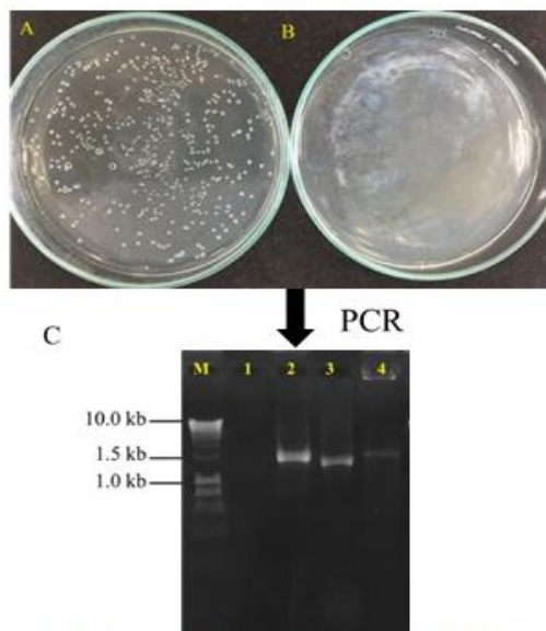
Fig. 3 Examination of the genetic transformation into A. tumefaciens .
