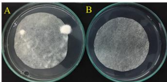
Fig. 4 Results of the co-cultivation process for the auxotrophic A. oryzae AUT1 strain.
